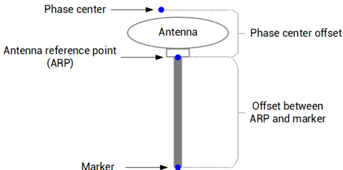
Figure 4-1 Schematic Diagram of the Antenna Phase Center and Antenna Reference Point
