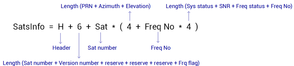
Figure 7-4 Explanation of the Binary Offset of SATSINFO
