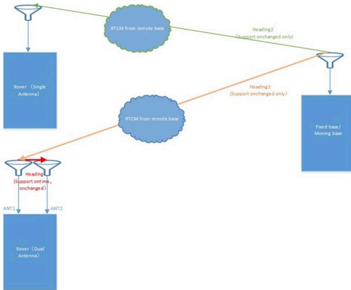
Figure 3-1 Heading Schematic
